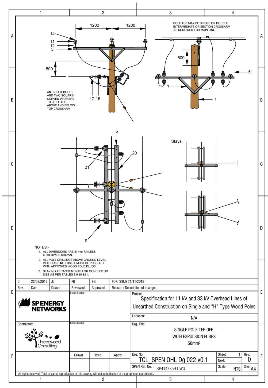
22.22 Figure 22 General Arrangement Single Pole Tee-off 50mm 2 with Expulsion Fuses (Drawing No. SP4147859)
